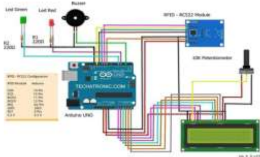
Fig 6 circuit diagram
